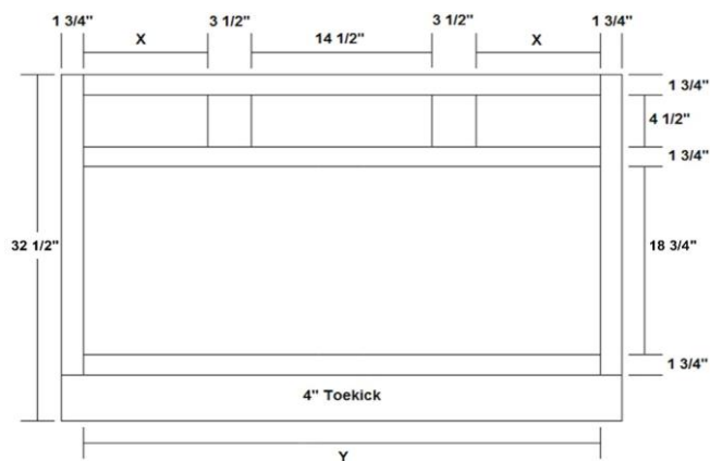
VANITY BASE W/ SIDE DRAWERS 36" - 45" WIDE
