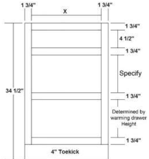
Base with Warming DWR and Two Working DWRS
