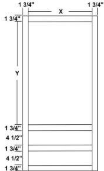
Standard Wall with Two Drawers
