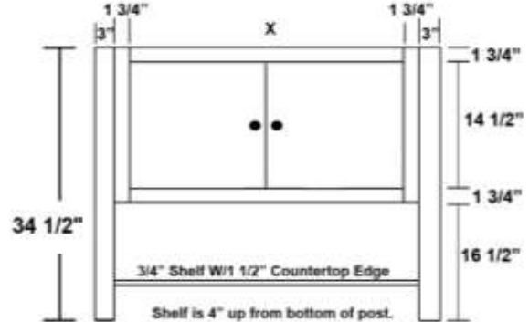
AH Vanity Furniture Base W/2 Doors
