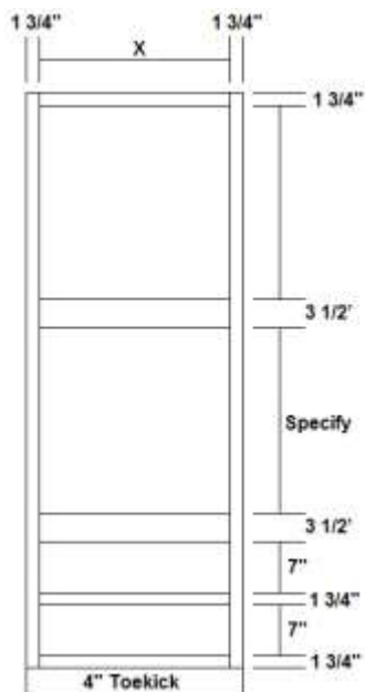
Single Oven Cabinet
