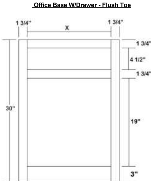
Opening Width Calculation Cabinet Width - 3.5" = X
