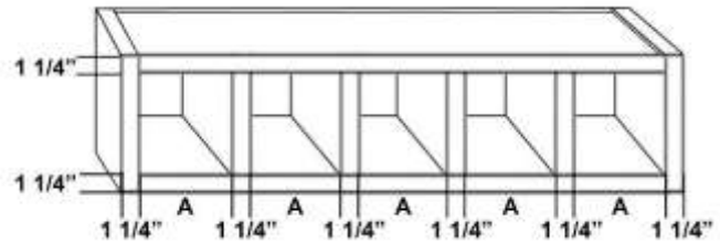
SHOWN - WWFF30X6.5X12H
