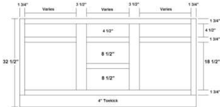
Vanity Base W/3 Center Drawers
