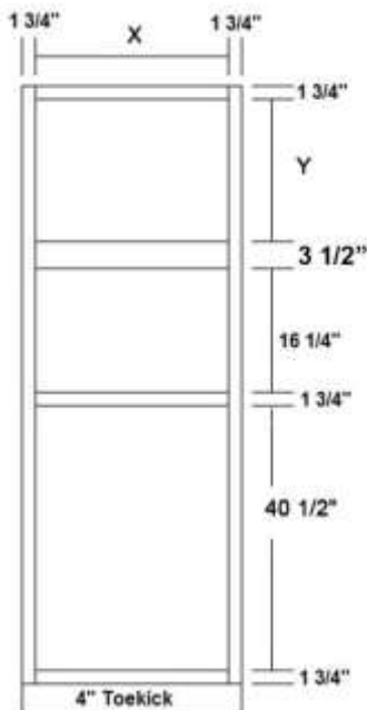
Microwave Oven Cabinet with doors
