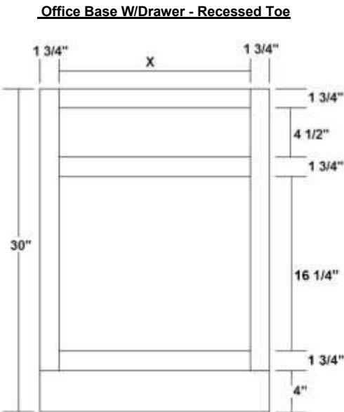
Opening Width Calculation Cabinet Width - 3.5" = X
