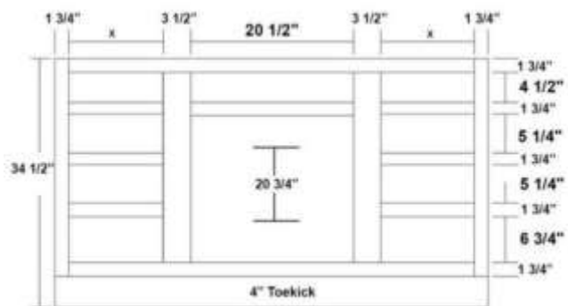
AH Vanity Base W/8 Double Drawers - 48" thru 72" Wide
