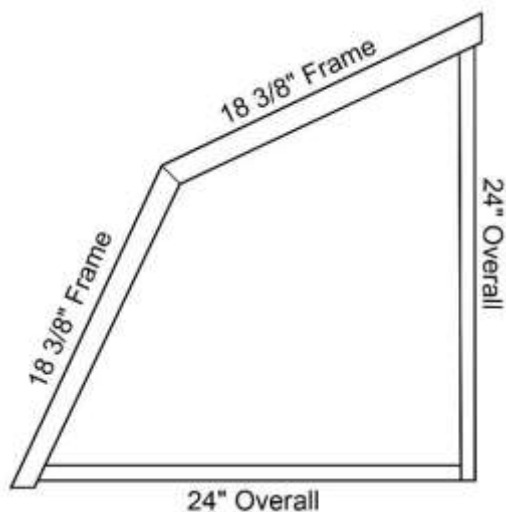
BA12U24U12
