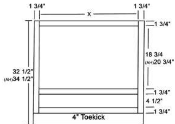
Inverted Sink Base with Two Drawers
