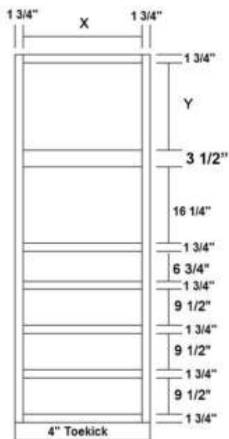
Microwave Oven Cabinet W/4 Drawers
