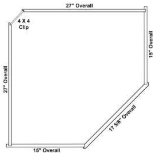
27W - 15" Deep Diagonal Wall Cabinets - Top View
