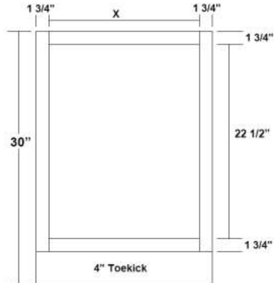
Office Base With Full Height Door - Recessed Toe
