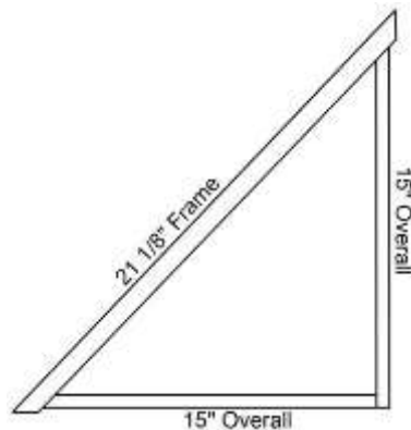
Diagonal Angle 15" Deep - Top View
