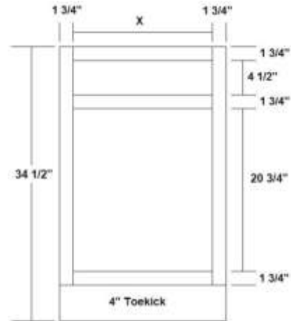
AH Vanity Base 12" to 39" wide
