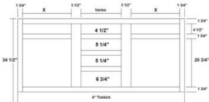
AH Vanity Base W/4 Center Drawers
