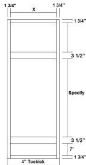
Double Oven Cabinet
