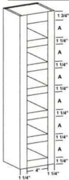
SHOWN - WWFF6.5X36X12V
