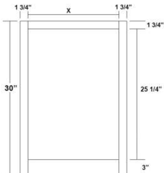
Office Base With Full Height Door - Flush Toe
