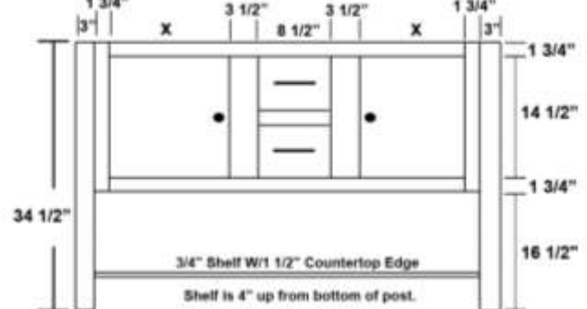
AH Vanity Furniture Base W/2 Doors & 2 Drawers
