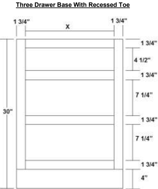
Opening Width Calculation Cabinet Width - 3.5" = X
