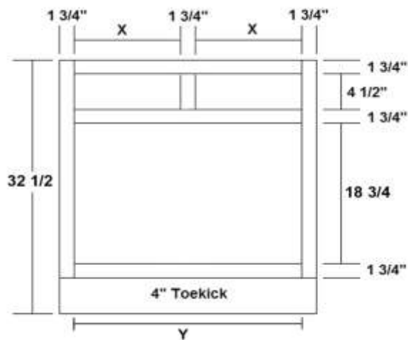
VANITY BASE 42" THRU 48" WIDE
