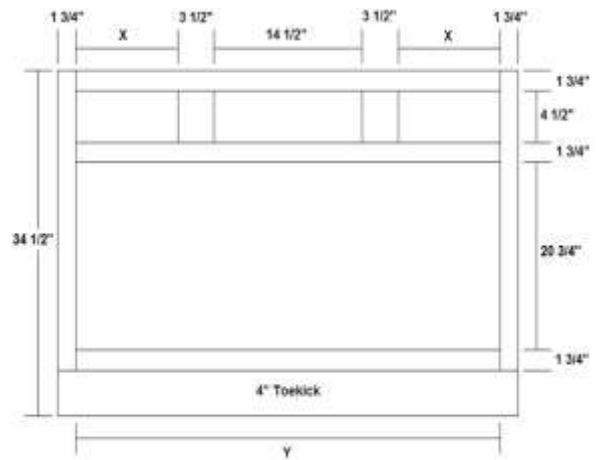
AH VANITY BASE W/ SIDE DRAWERS 36" - 45" WIDE
