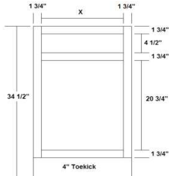
AH VANITY BASE 12" THRU 39" WIDE
