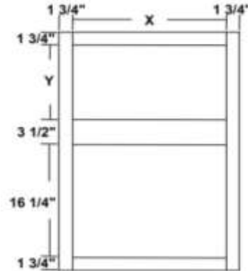
BUILT IN MICROWAVE CABINET 36" THRU 42" TALL
