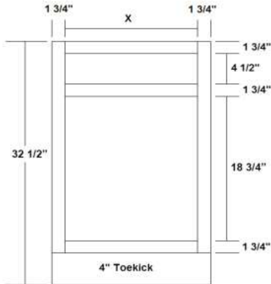
VANITY BASE 12" THRU 39" WIDE
