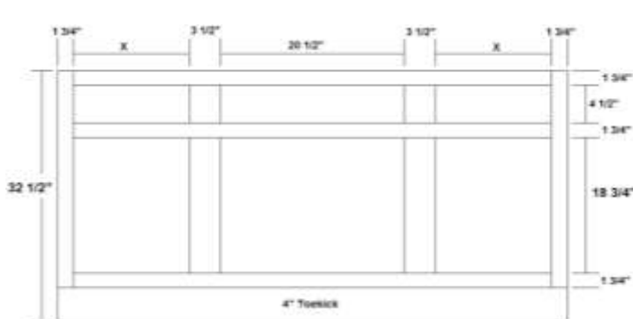
VANITY BASE W/ SIDE DRAWERS 48" - 60" WIDE
