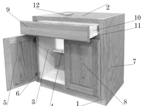
BASE CABINET
