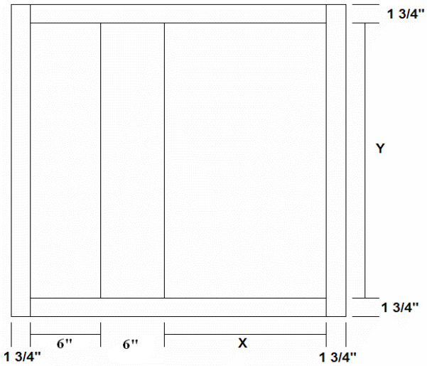
WALL BLIND CORNER W/ONE DOOR OR TWO BUTT DOORS
