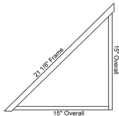
DIAGONAL ANGLE 15" DEEP - TOP VIEW
