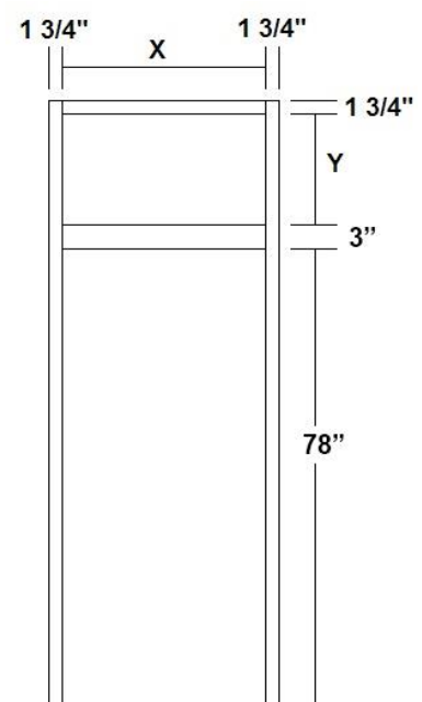
90", 93", & 96" WALK THRU PANTRY
