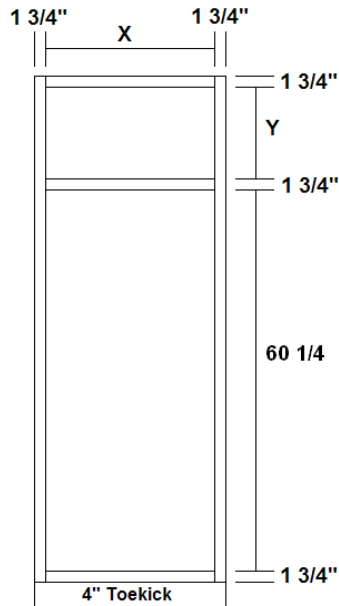
PANTRY
