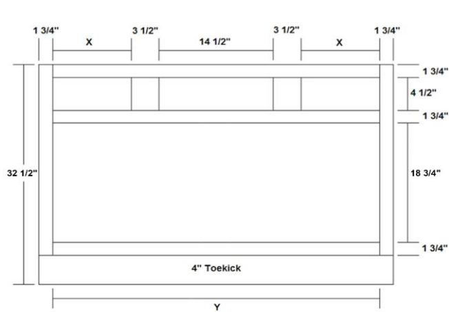
VANITY BASE W/ SIDE DRAWERS 36" - 45" WIDE
