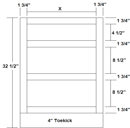
VANITY DRAWER BASE
