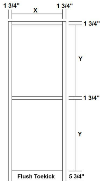
LINEN FRONT
