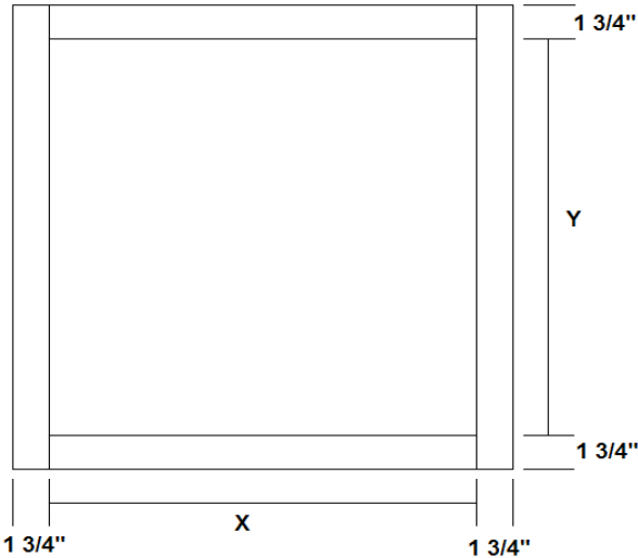
STANDARD WALL W/ONE DOOR OR TWO BUTT DOORS
