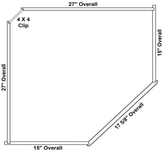
27" WIDE - 15" DEEP DIAGONAL WALL CABINETS - TOP VIEW
