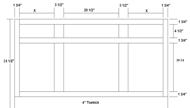
AH VANITY BASE W/ SIDE DRAWERS 48" - 60" WIDE
