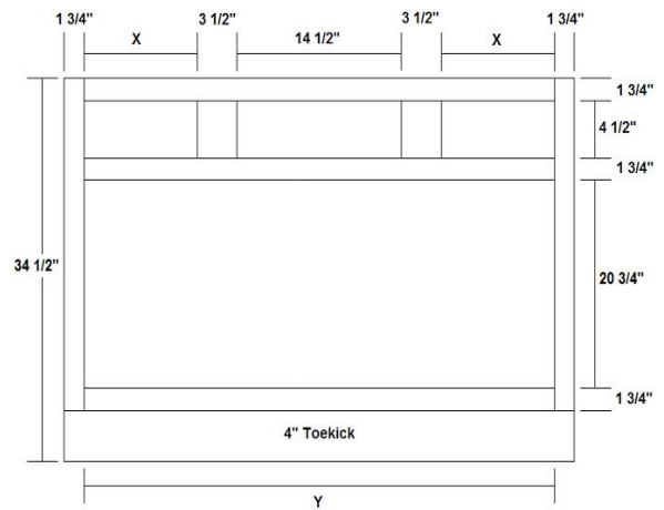
AH VANITY BASE W/ SIDE DRAWERS 36" - 45" WIDE
