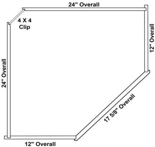
24" WIDE - 12" DEEP DIAGONAL WALL CABINETS - TOP VIEW
