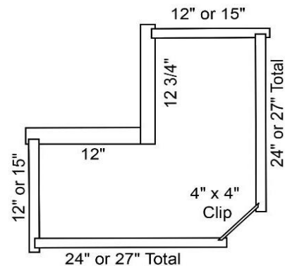
12" & 15" DEEP WALL EASY REACH TOP VIEW
