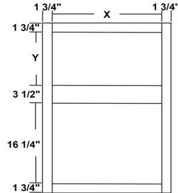
BUILT IN MICROWAVE CABINET 36" THRU 42" TALL
