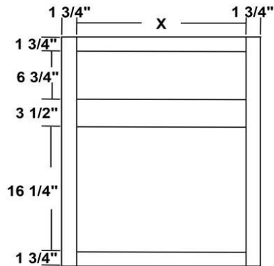
BUILT IN MICROWAVE CABINET 30" TALL
