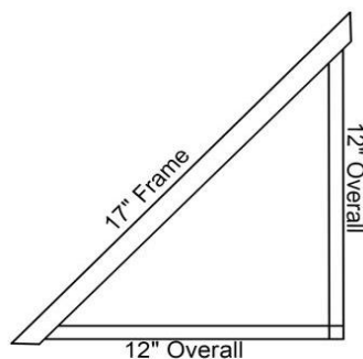
DIAGONAL ANGLE 12" DEEP - TOP VIEW
