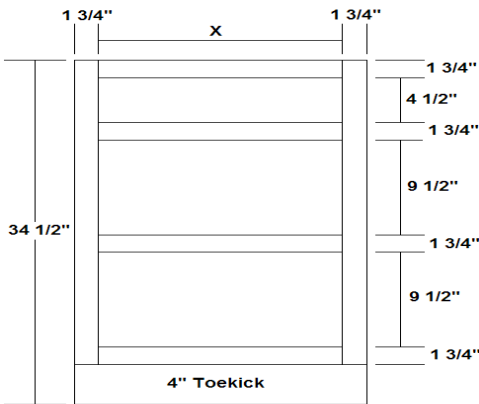
AH VANITY DRAWER BASE
