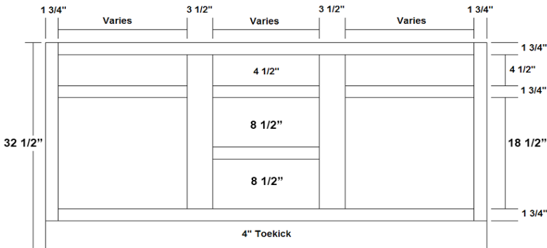
AH VANITY BASE WITH CENTER DRAWERS
