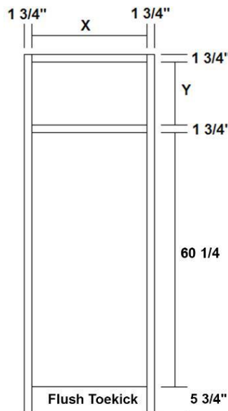
PANTRY FRONT
